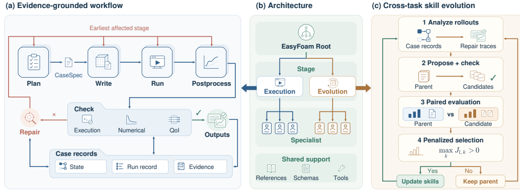
Figure 2: Overview of EasyFoam. (a) Execution loop: evidence-guided construction and stage-scoped repair. (b) Architecture: hierarchical skill organization. (c) Evolution loop: experience distillation via paired evaluation.
