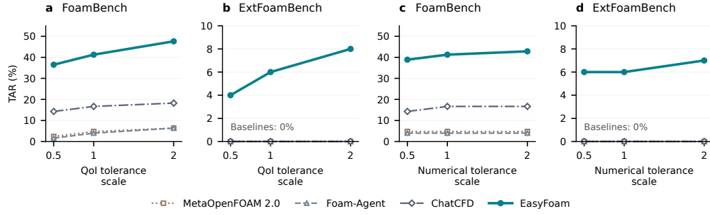
Figure 3: TAR sensitivity to QoI tolerances (a,b) and Numerical tolerances (c,d) on FoamBench (a,c) and ExtFoamBench (b,d). The three baselines in (b,d) overlap at zero.
