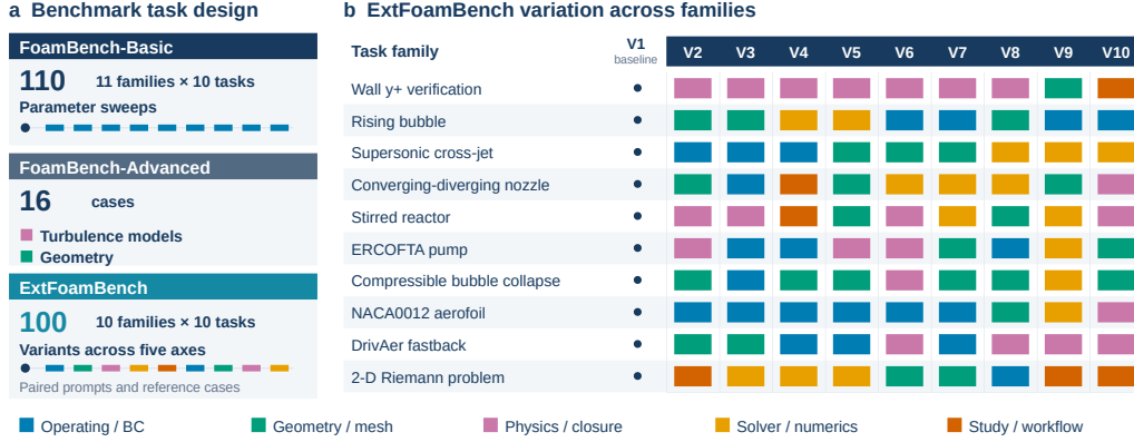
Figure 1: Task construction and variation in FoamBench and ExtFoamBench. (a) FoamBench-Basic primarily uses parameter sweeps, while FoamBench-Advanced contains 16 cases with variation concentrated in turbulence models and geometry. ExtFoamBench contains ten families, each with one baseline and nine variants. (b) Colors indicate the primary variation axis of each variant.
